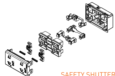
SAFETY SHUTTER
