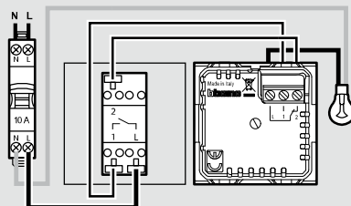
Two-way switch + Two-way energy saving switch
