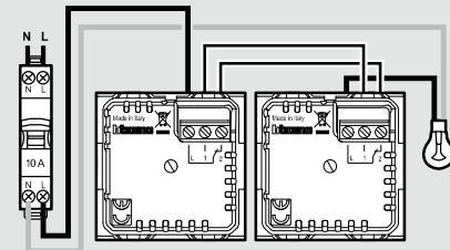
2 Two-way energy saving switches
