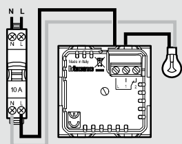
Two-way energy saving switch
